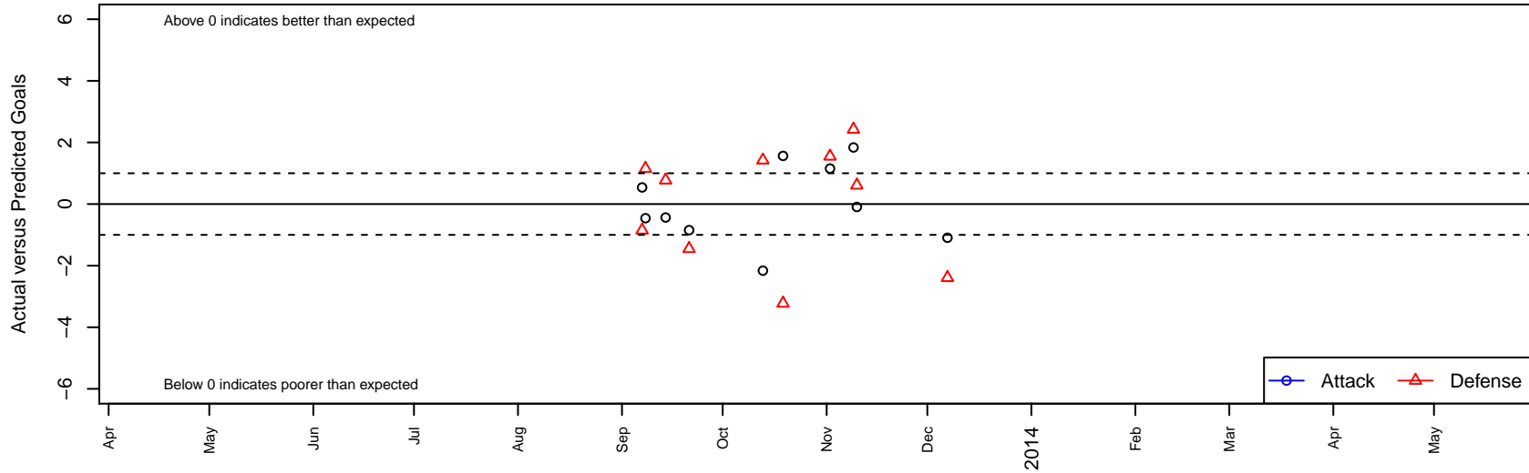
SRU AC Milan B01 Dots are actual minus expected GF (blue circles) and GA (red triangles). Blue line is smoothed change in attack strength. Red is smoothed change in defense strength.
